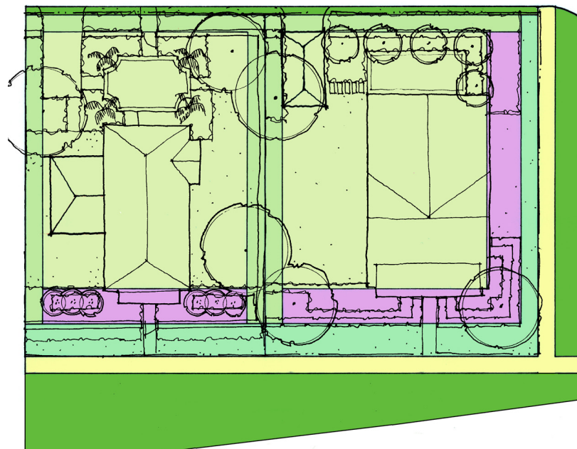
Plan of typical house placement on the Golf View lots
